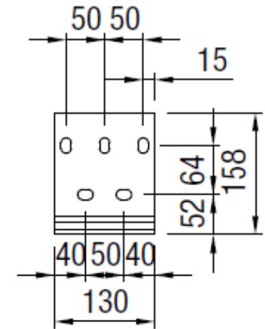
BRACKET PLATE FOR STD. WALL INSTALLATION
