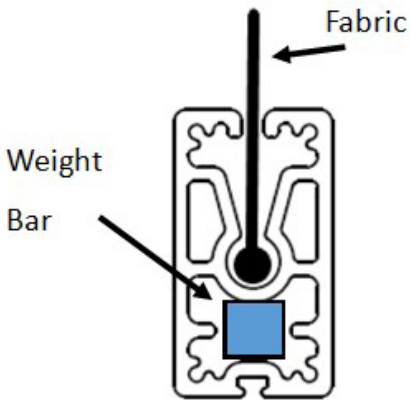
Hem bar: Side view
