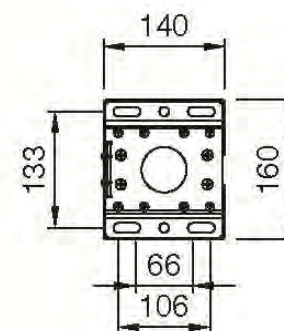
FOOT PLATE
