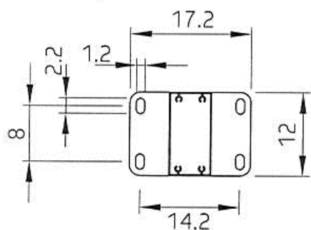
Ground plate
