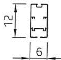
Crossbar profile cod. 2799
