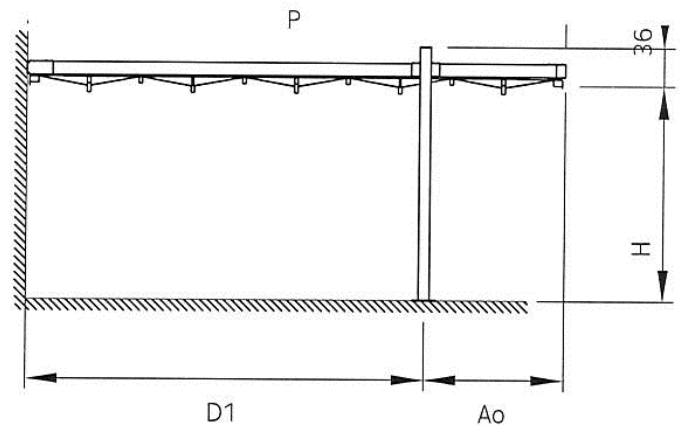
Rear mounting with arched wall
