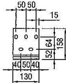
BRACKET PLATE FOR STANDARD WALL INSTALLATION
