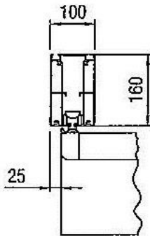
FRONT SECTION
