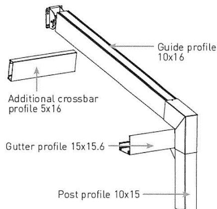
Version with gutter
