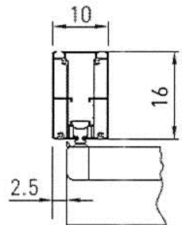
Front section
