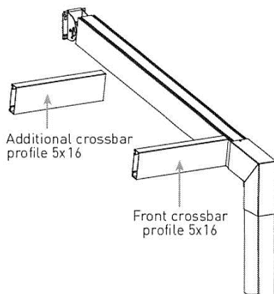
Version with crossbar front profile
