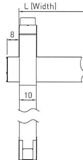
Front section
