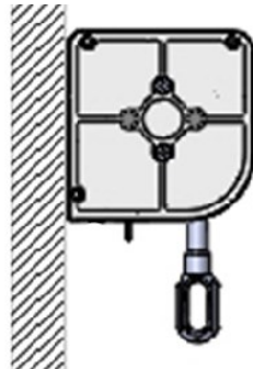
Front standard gear loop.
