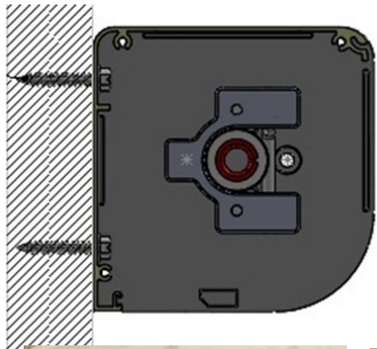
Ceiling or wall mounting cassette possible.
