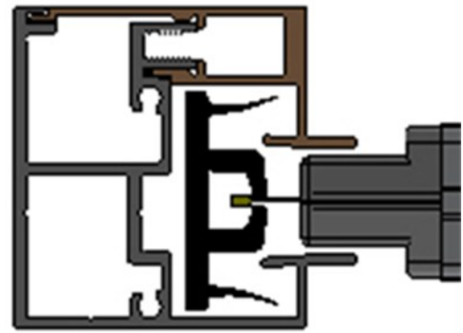
Standard track with zipper and track assembly.
