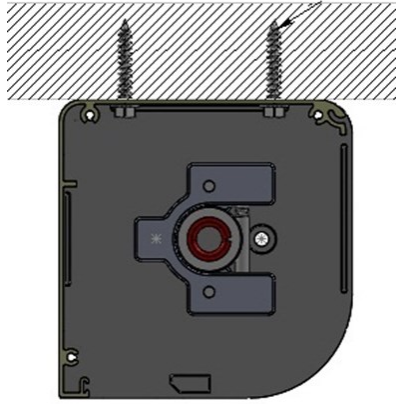
Ceiling or wall mounting cassette possible.
